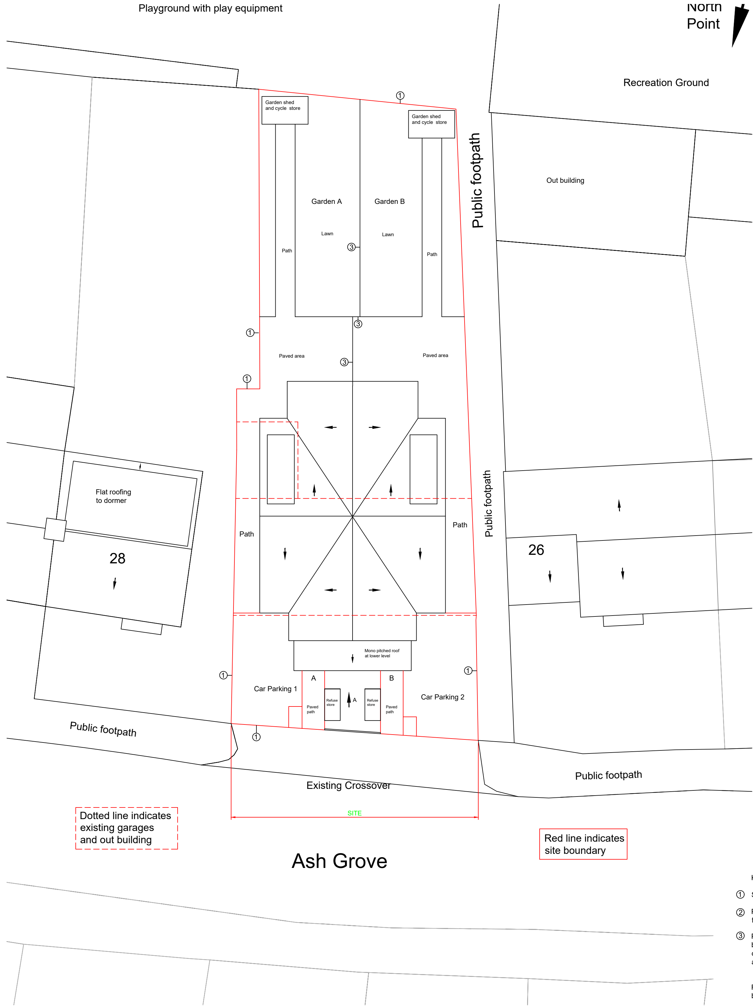
Proposed Site Block Plan Scale 1:100
