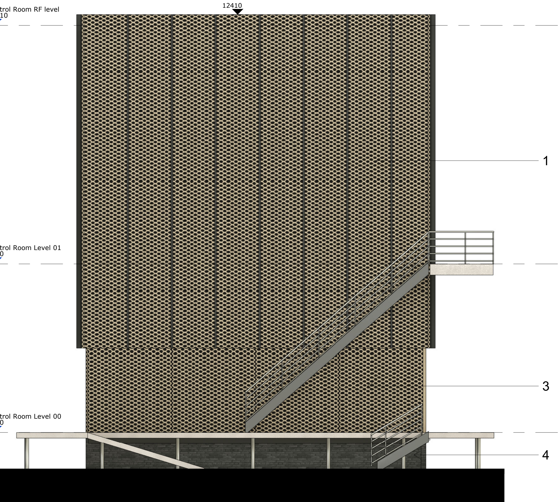
Control Room - South Elevation 1 : 50
