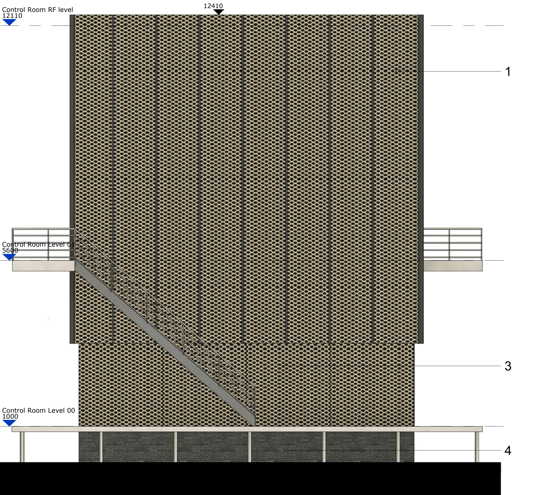
Control Room - North Elevation 1 : 50
