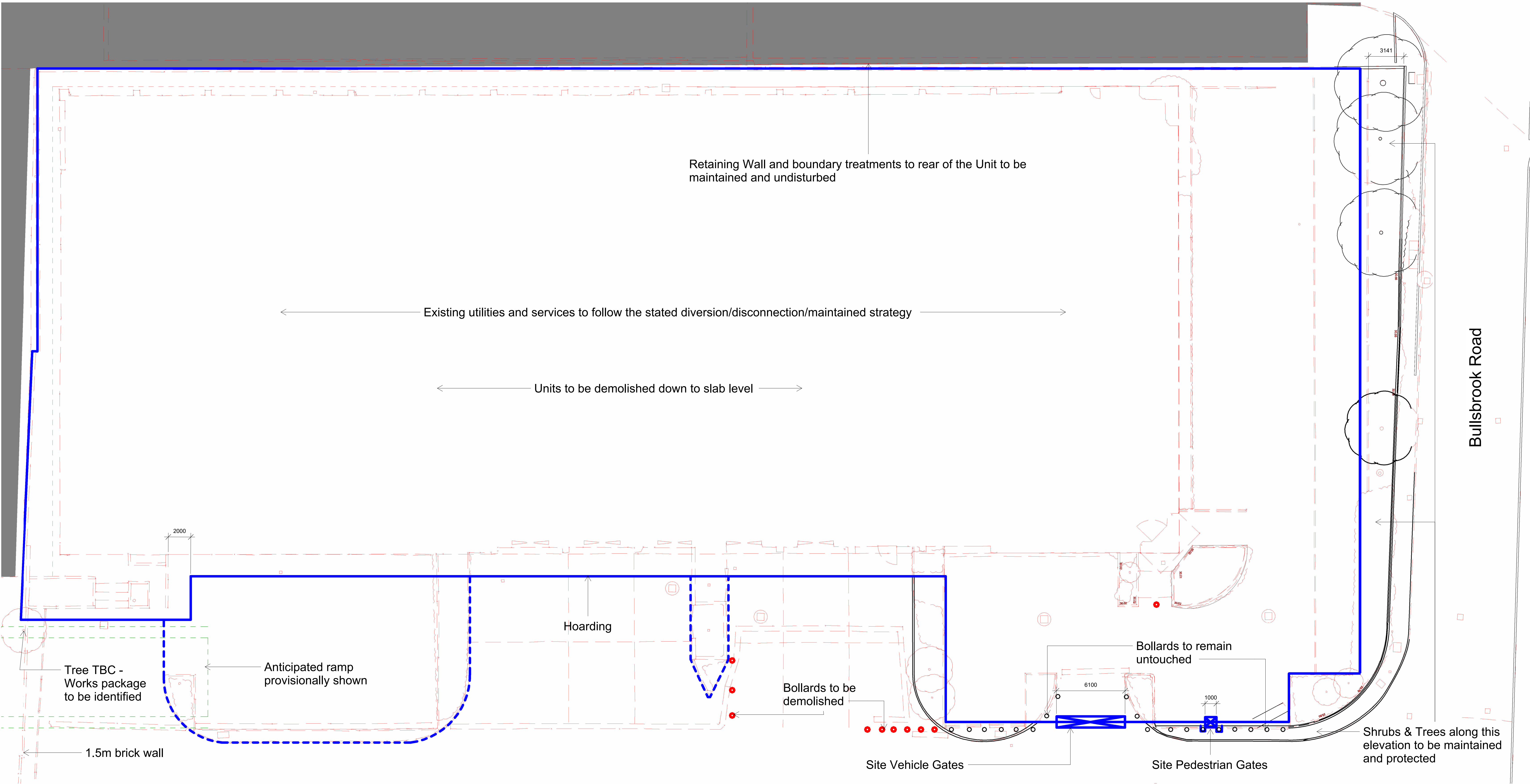
Demolition Ground Level Plan 1 : 150
