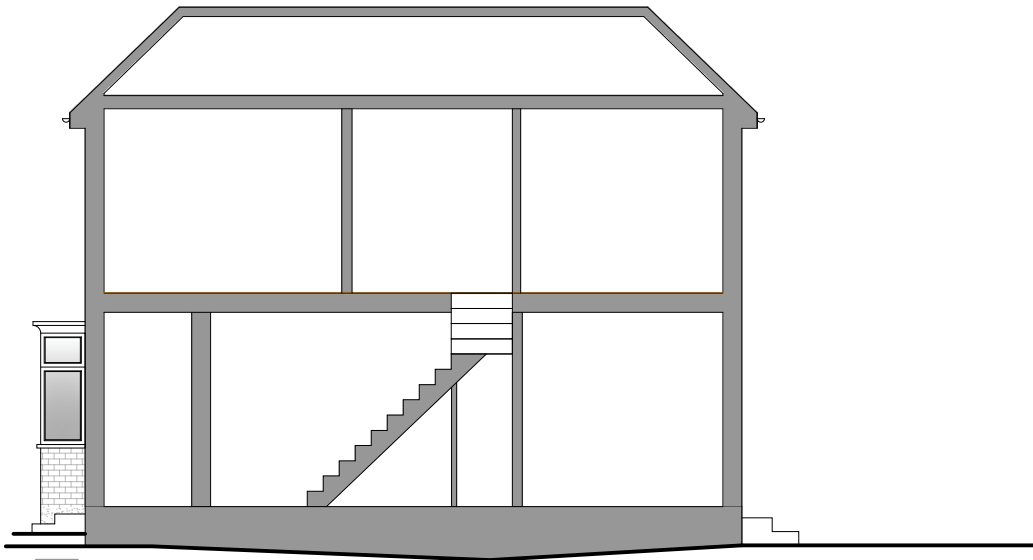
7 Existing Side Section
