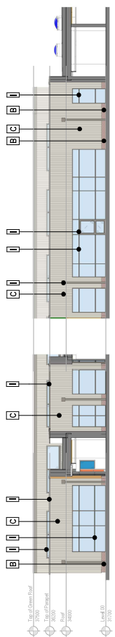
1 Low-stimulus building, internal courtyard 1 : 100
