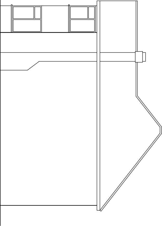
EXISTING SIDE ELEVATIONS (VIEW FROM NO. 29) SCALE 1:100
