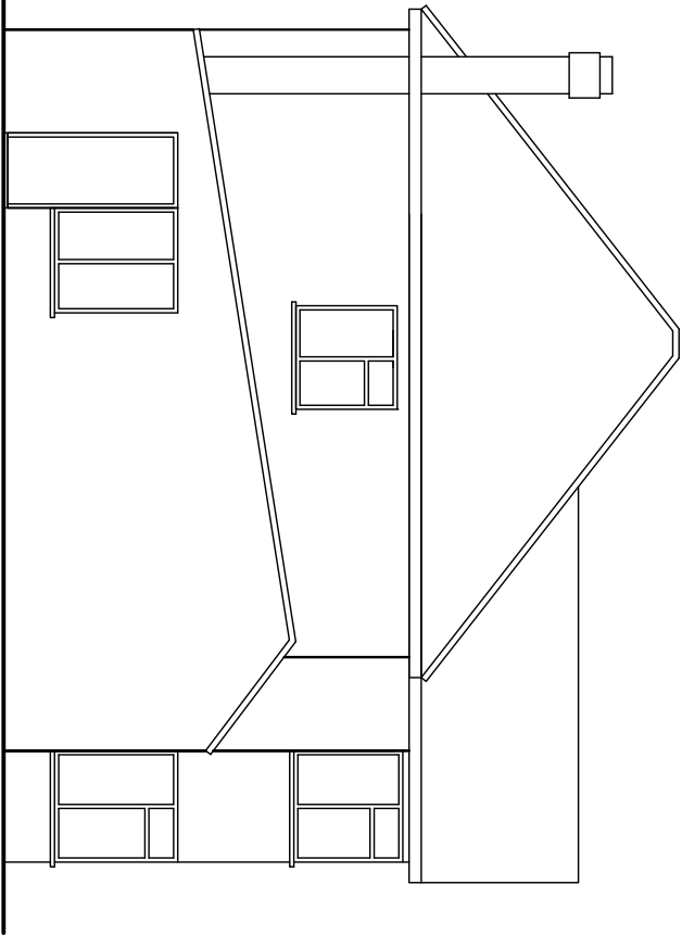
EXISTING SIDE ELEVATIONS (VIEW FROM NO. 25) SCALE 1:100
