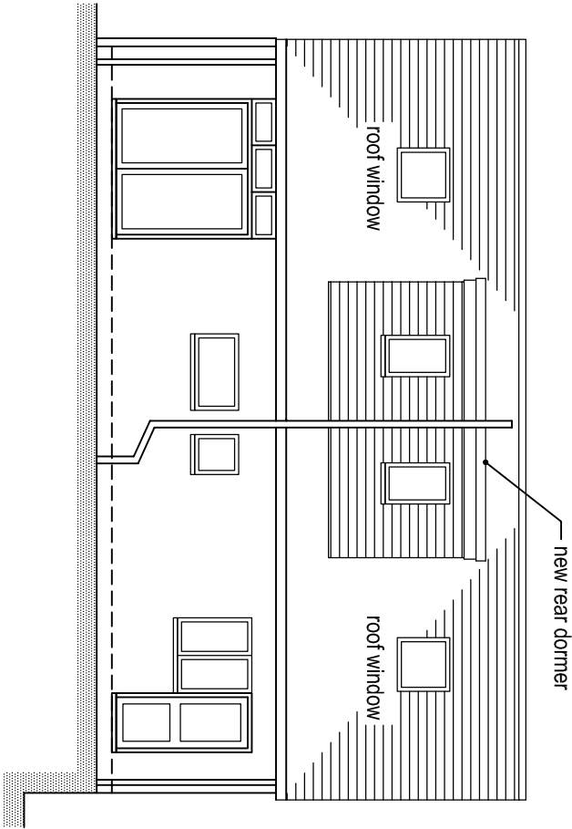
south elevation
