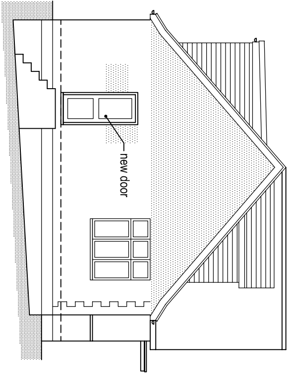
east elevation
