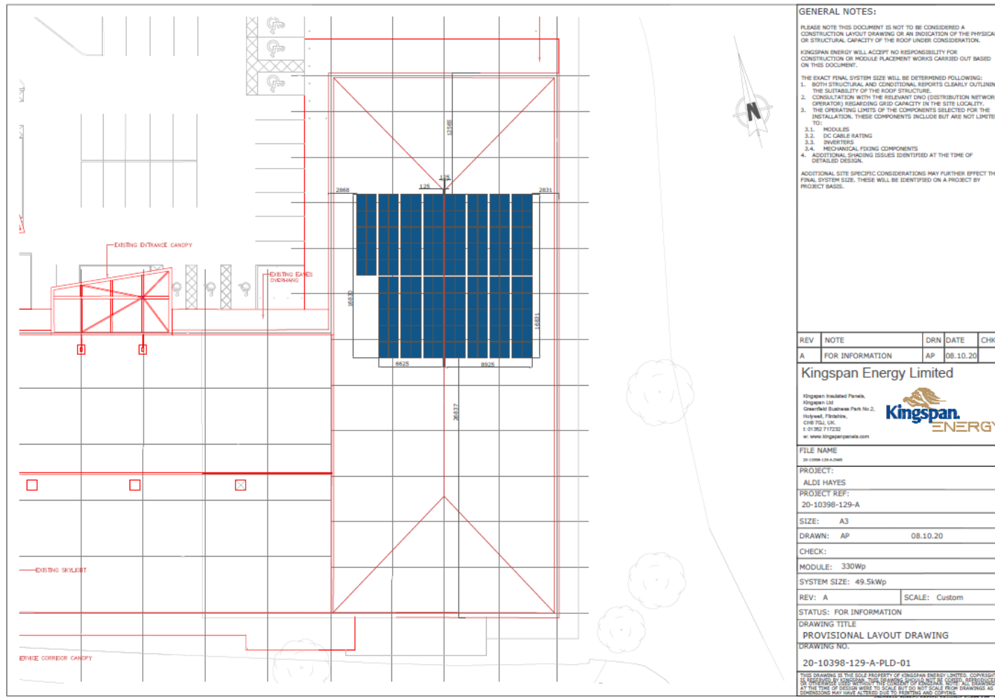
Figure ES1 Proposed PV Layout (prepared by Kingspan Energy)
