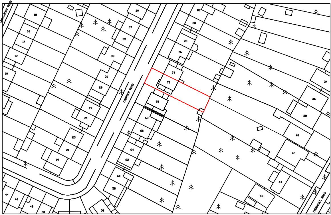
LOCATION PLAN (1:1250)
