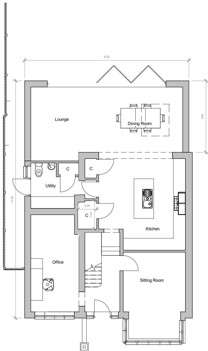
Ground floor 1 : 100
