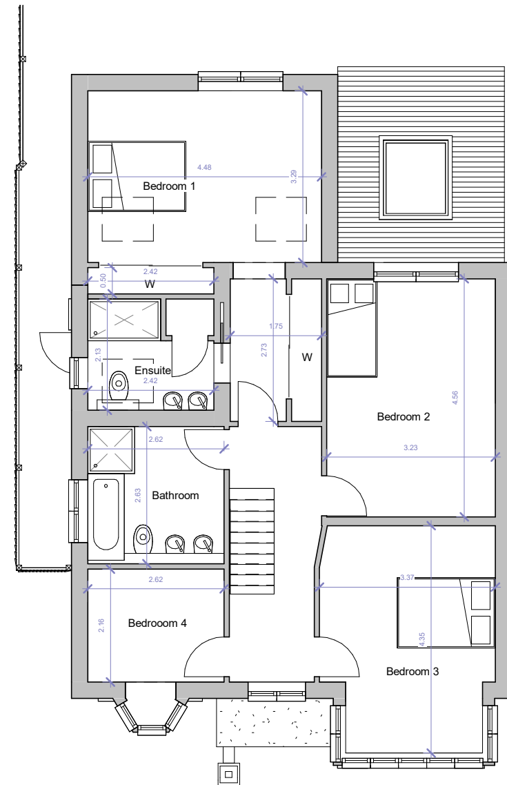
First floor 1 : 100
