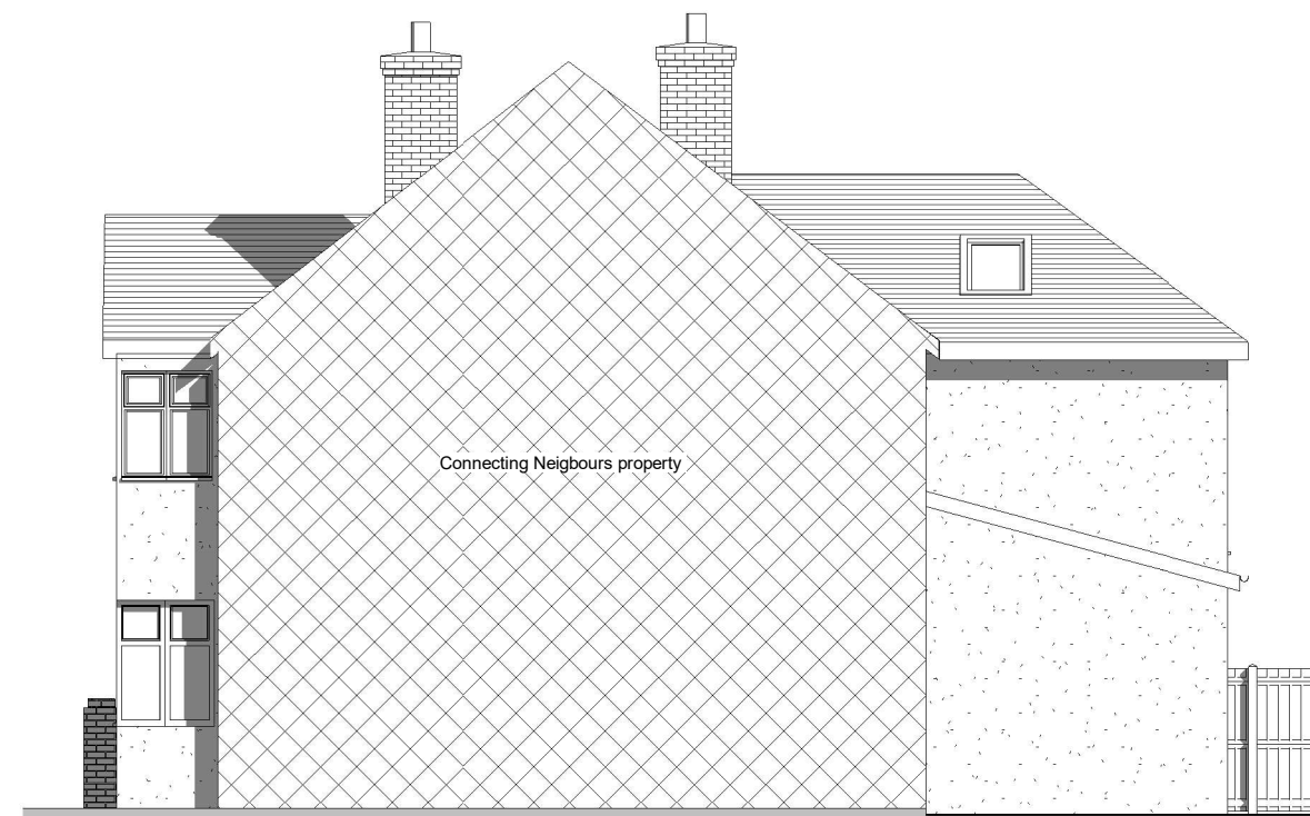
Proposed Side 2 Elevation 1 : 100
