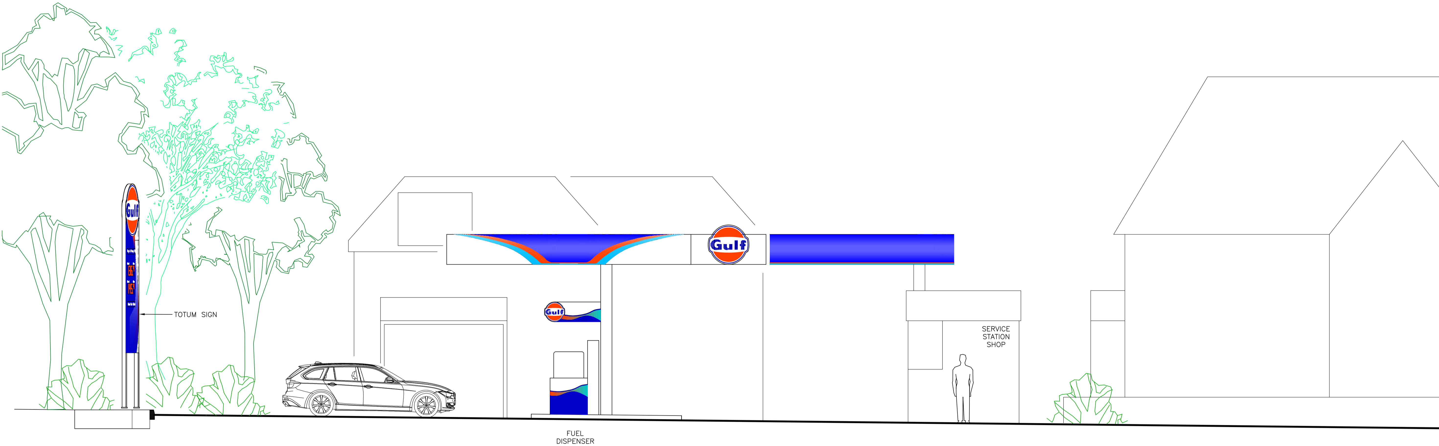
VIEW FROM ARROW A SCALE 1:50
