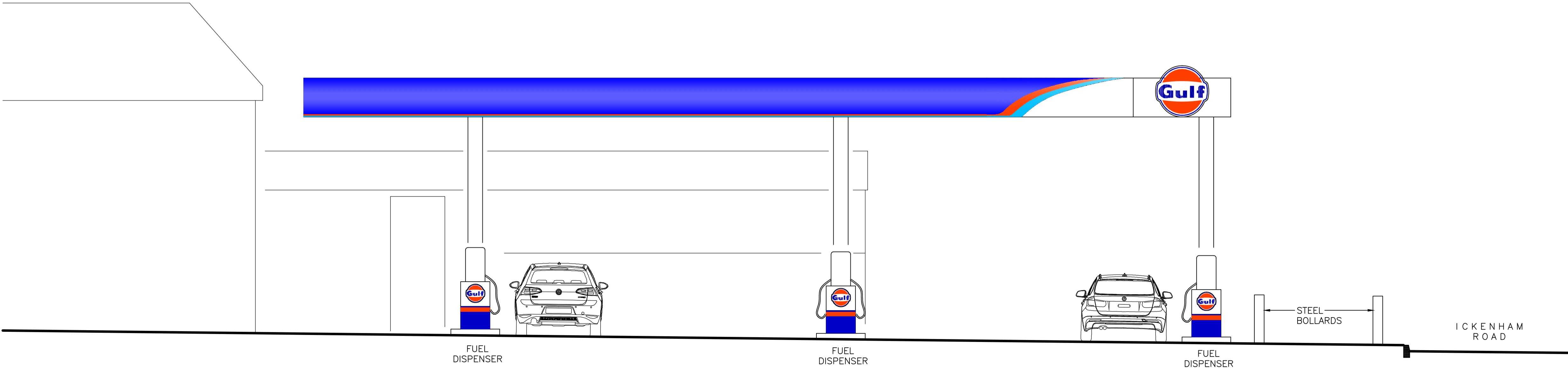
VIEW FROM ARROW B SCALE 1:50
