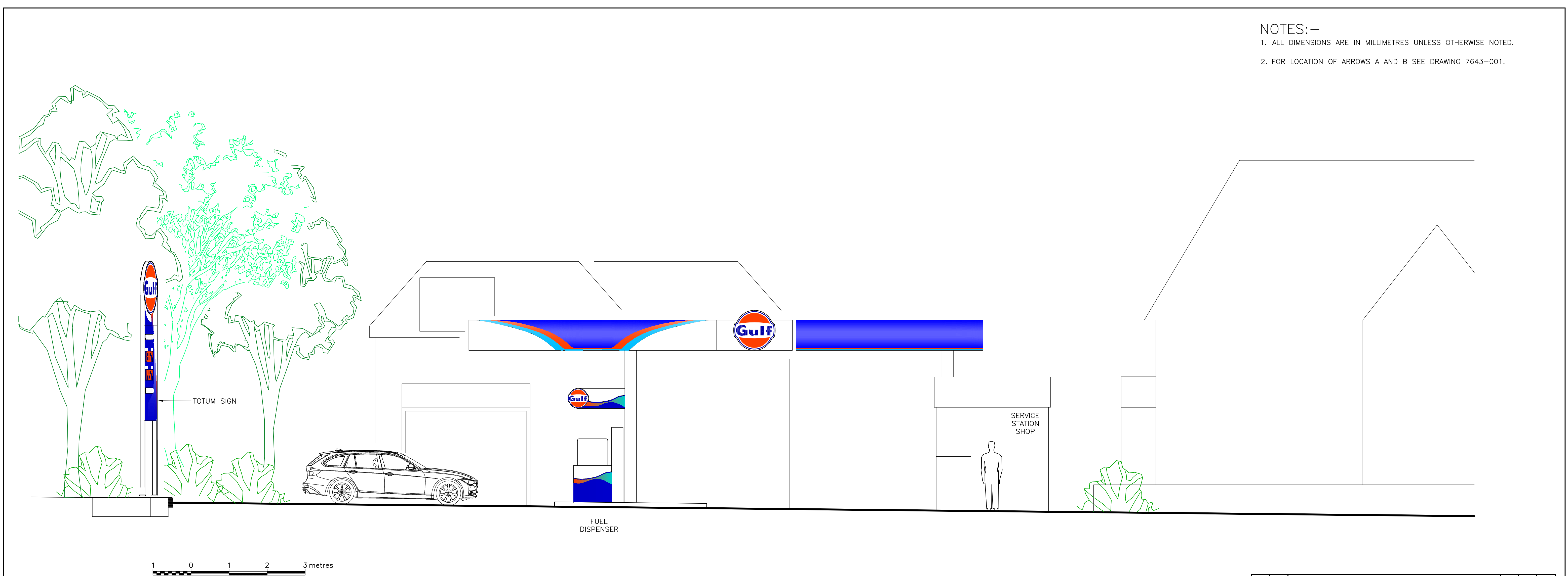
VIEW FROM ARROW A SCALE 1:50
