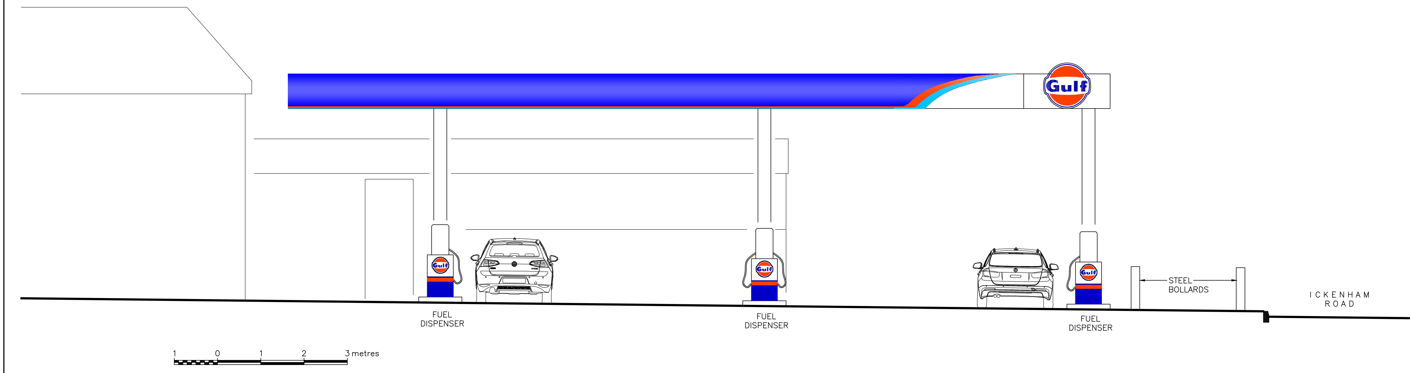
VIEW FROM ARROW B SCALE 1:50
