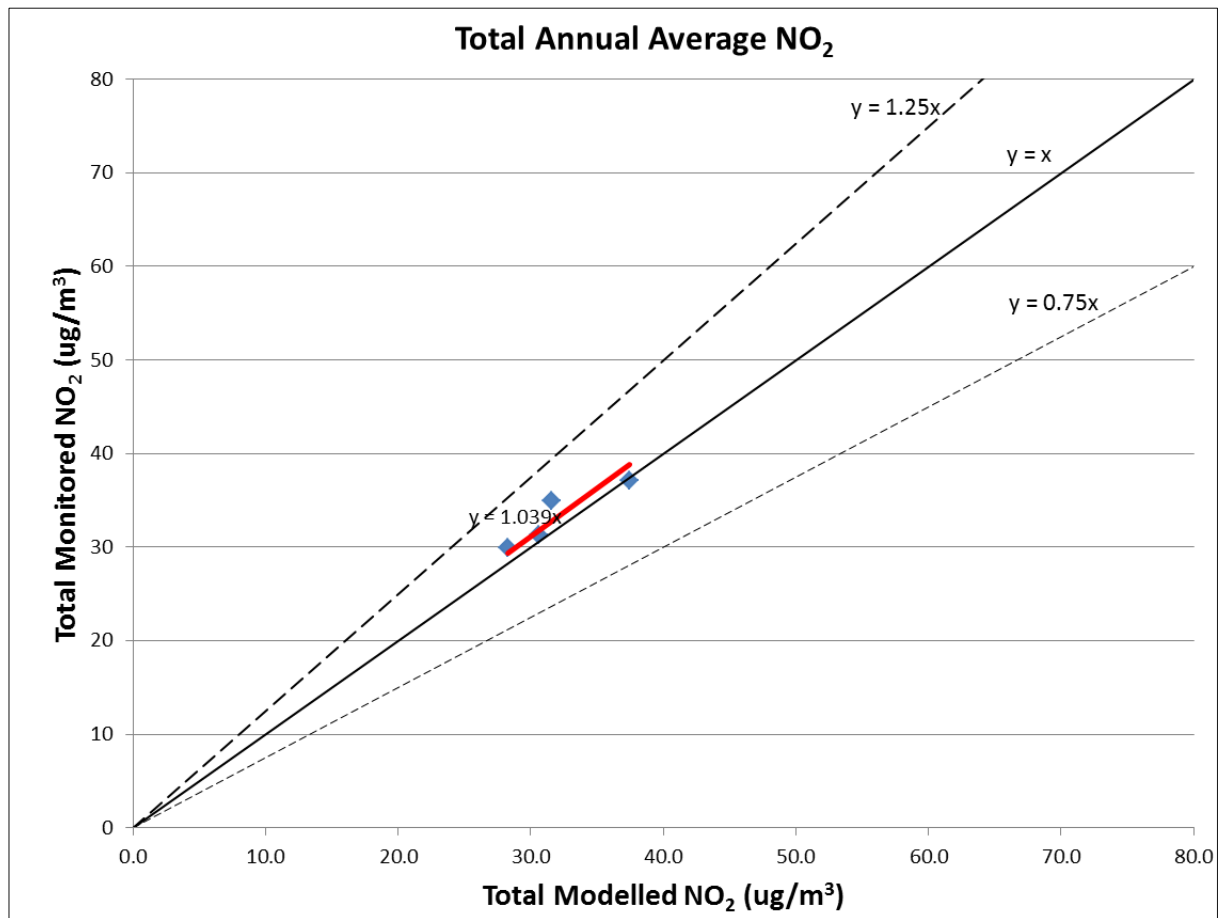
Figure 3-1 Comparison between modelled and monitored total NO 2
