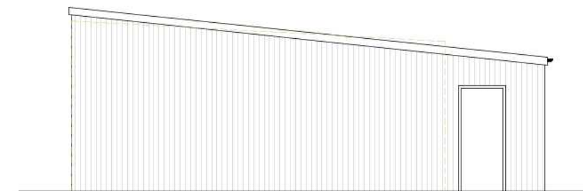
PROPOSED SIDE ELEVATION 1:100
