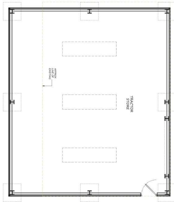
PROPOSED GROUND FLOOR PLAN 1:100
