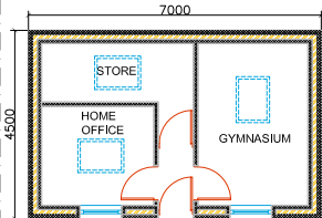
PROPOSED OUT-BUILDING
