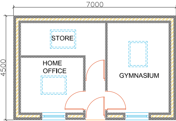
PROPOSED OUT-BUILDING
