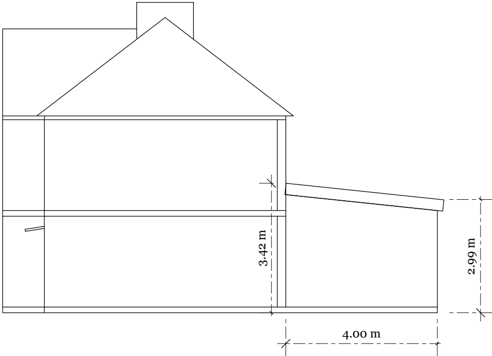
RIGHT PROPOSED (section)
