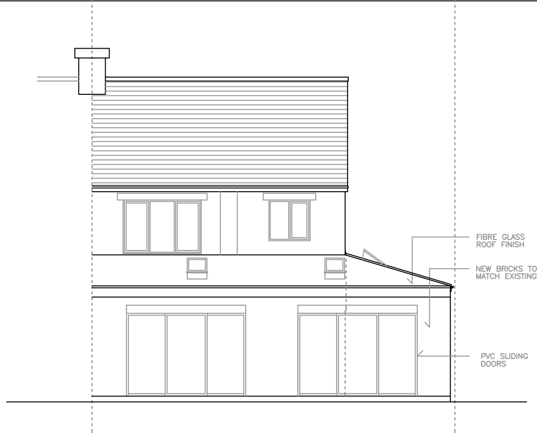
EXISTING BACK ELEVATION
