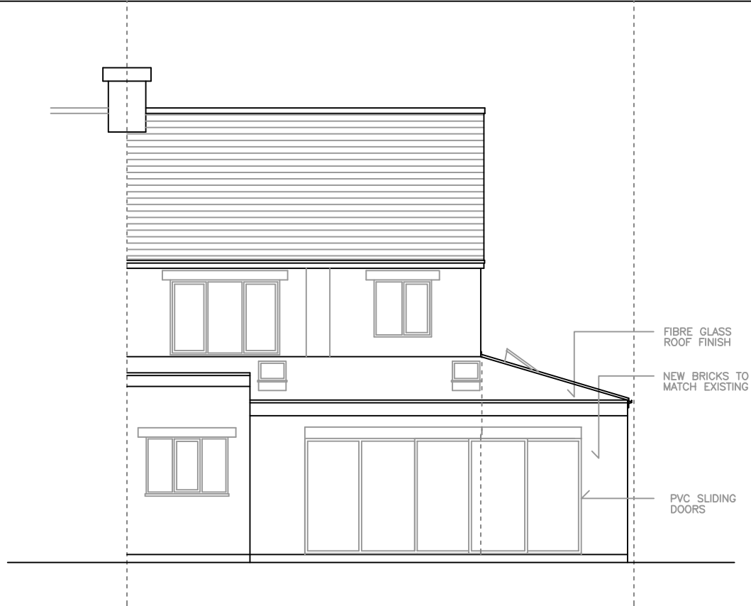
PROPOSED BACK ELEVATION
