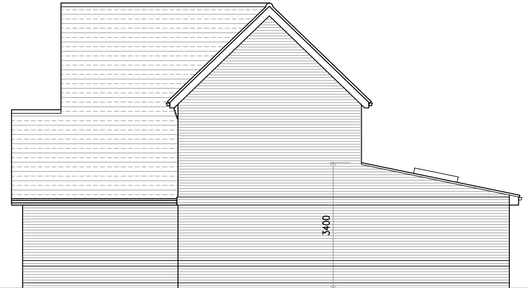
SIDE ELEVATION FACING NO. 12
