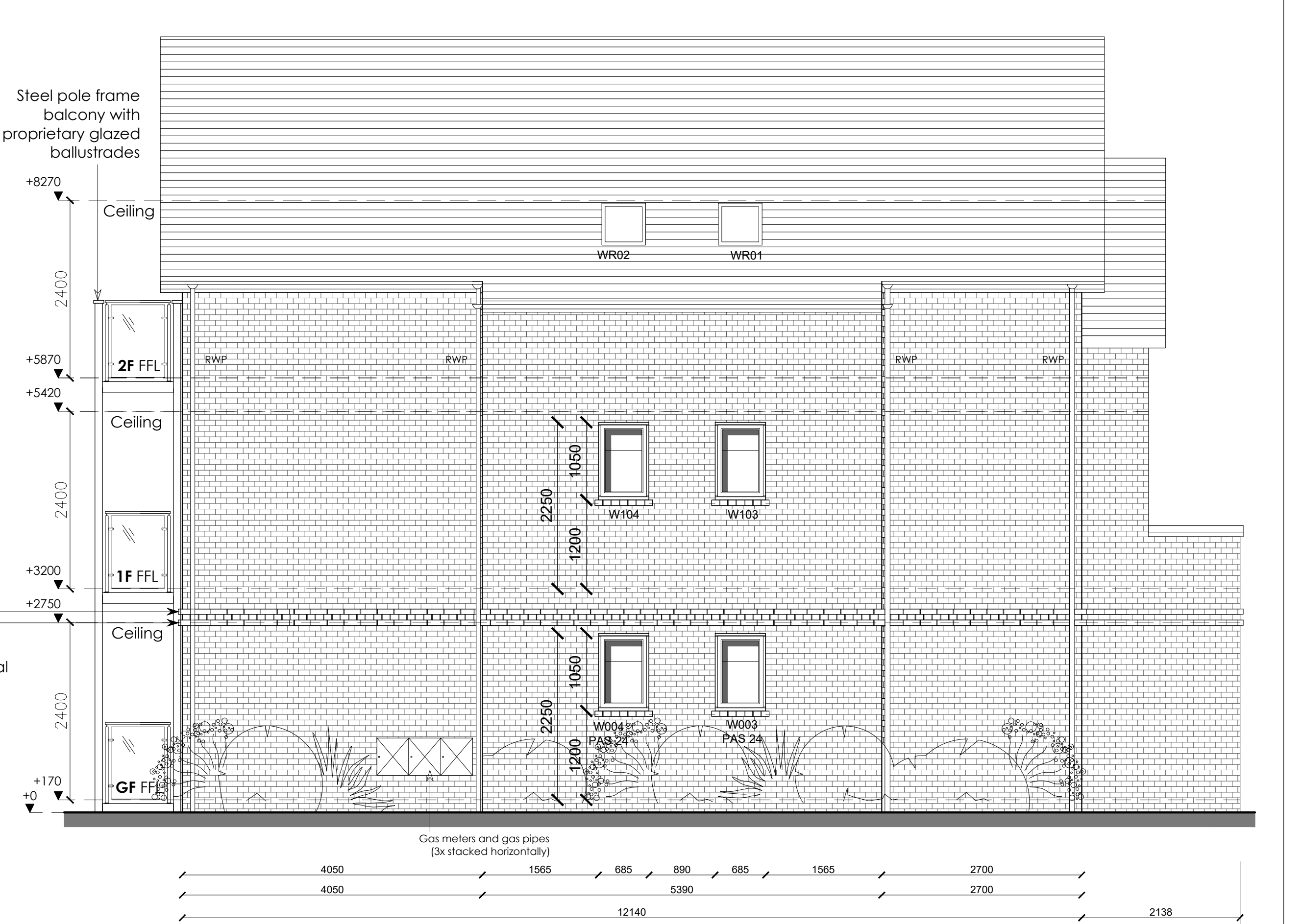
South Elevation
