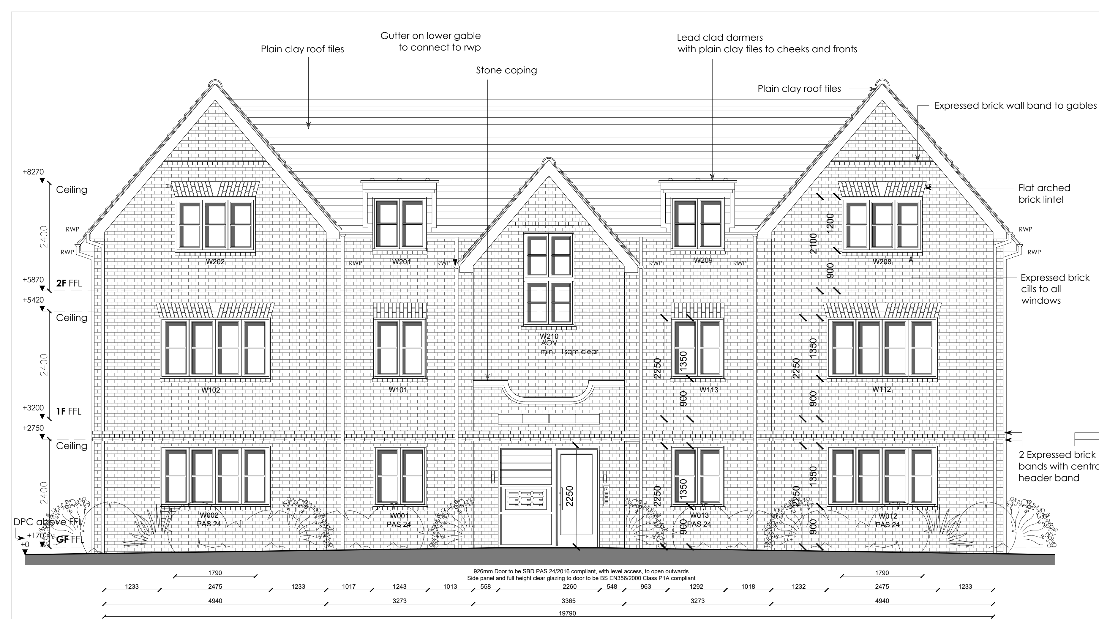
East Elevation
