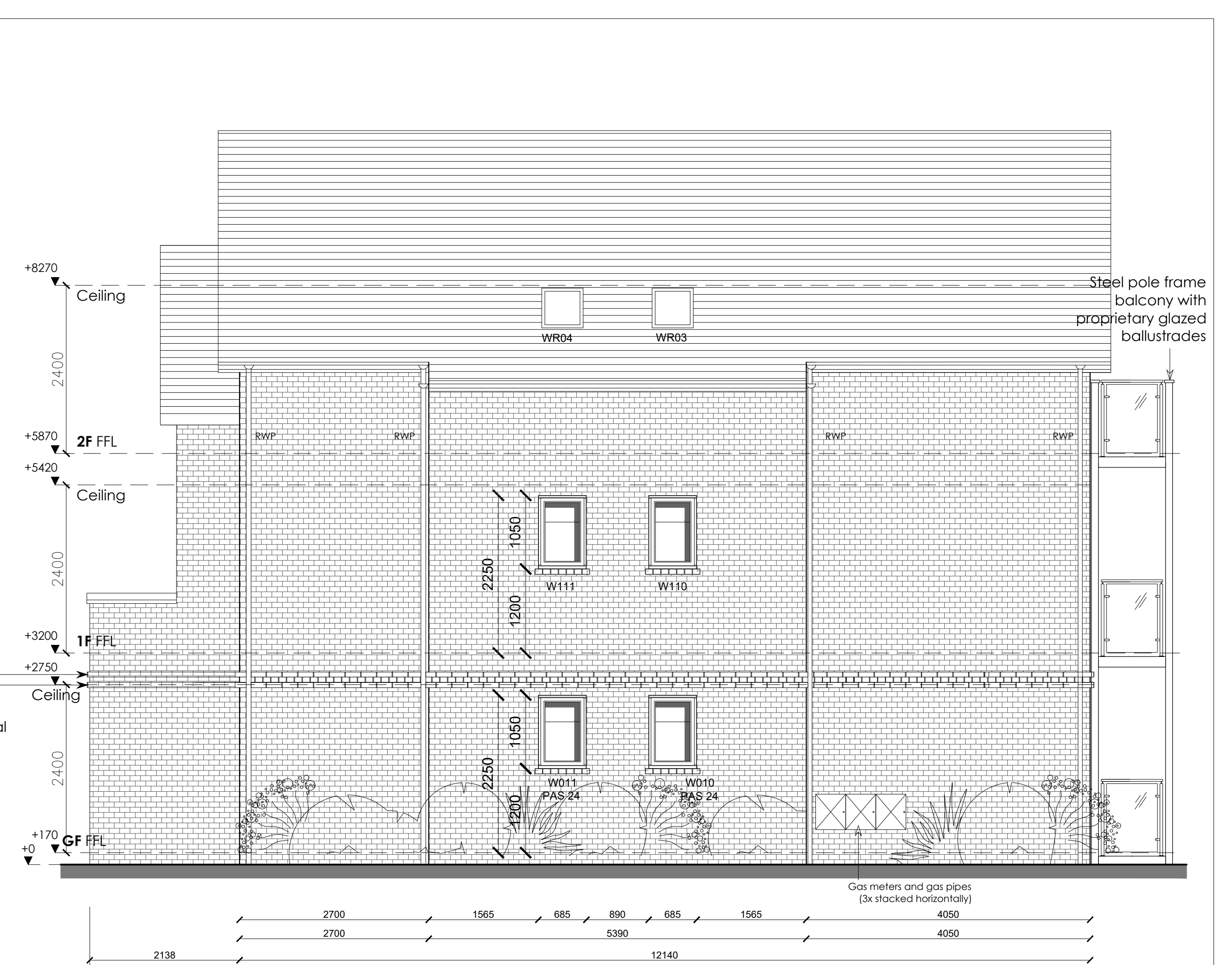
North Elevation
