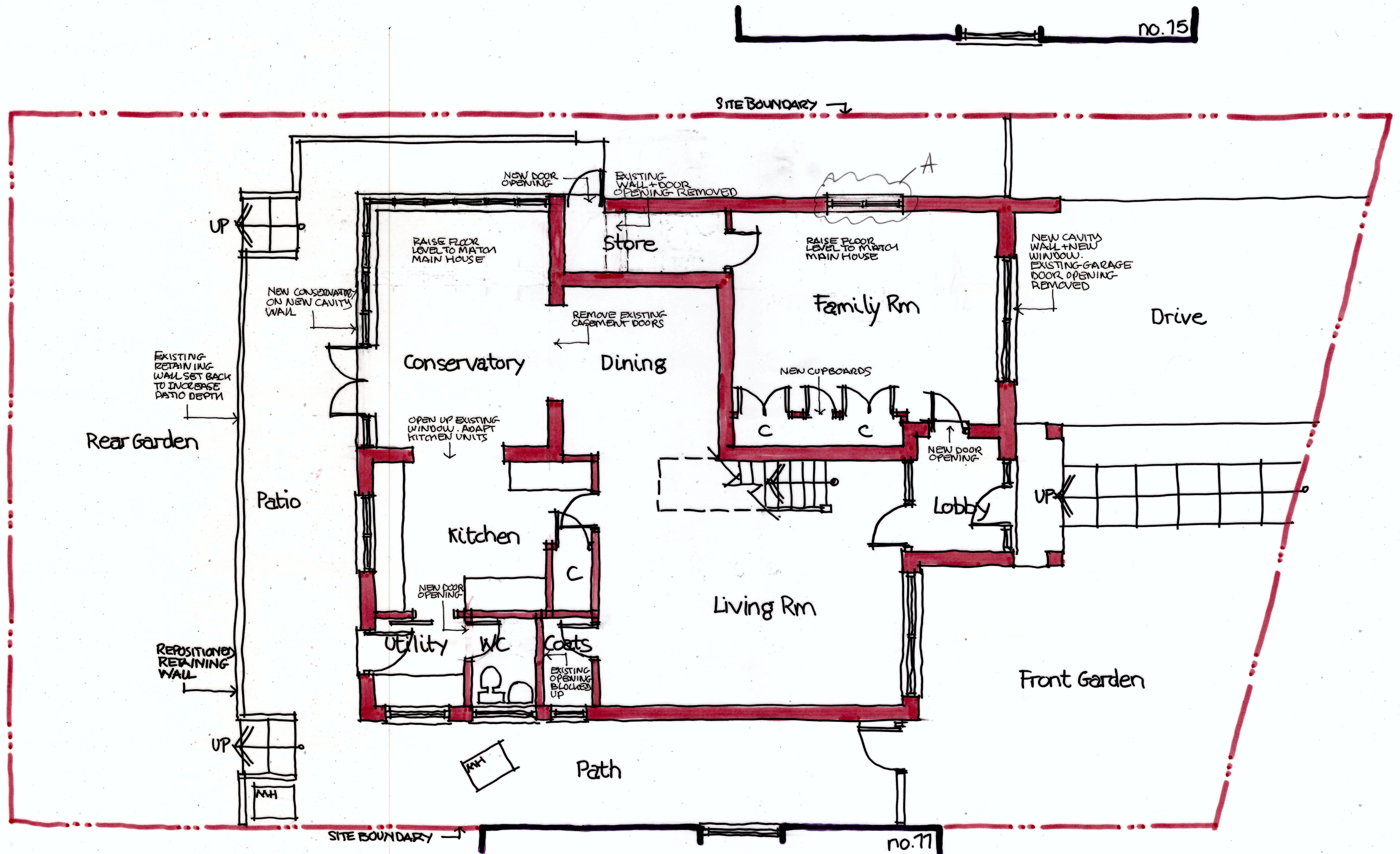
Proposed Ground Floor Plan 1:50 © A2
