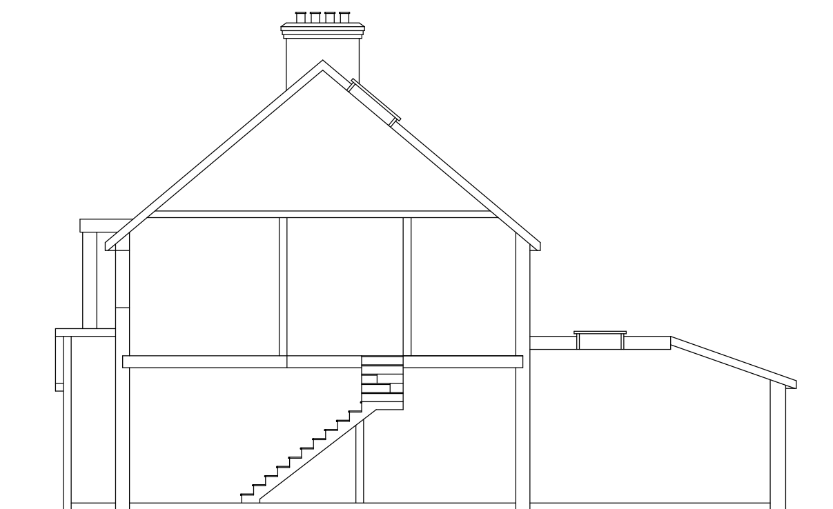
Existing Right Side Section
