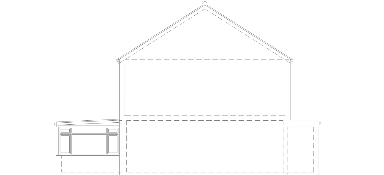
Side East Elevation Existing
