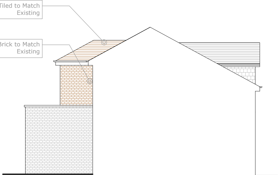
8 Proposed Side Elevation
