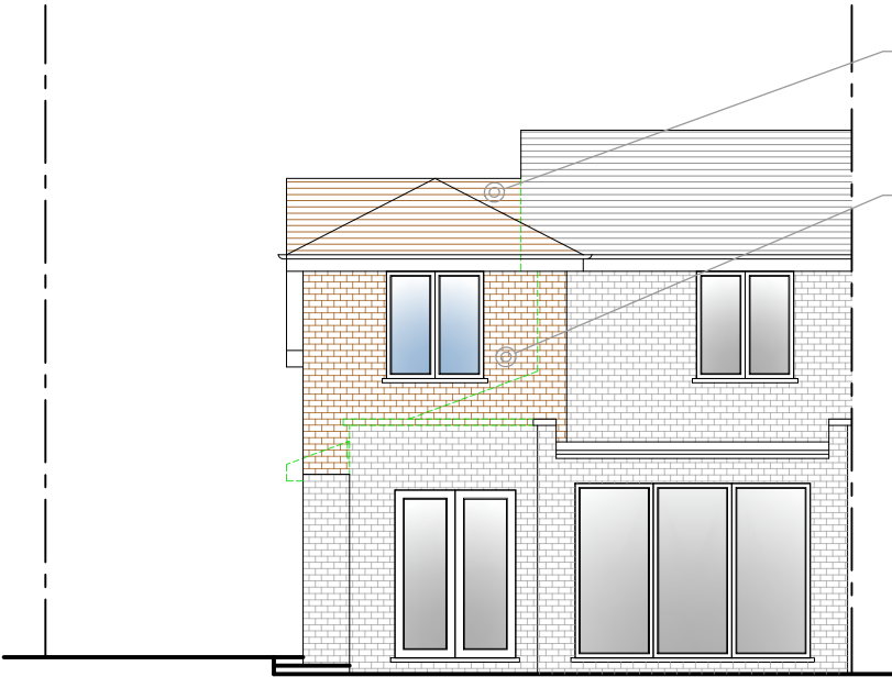
7 Proposed Rear Elevation
