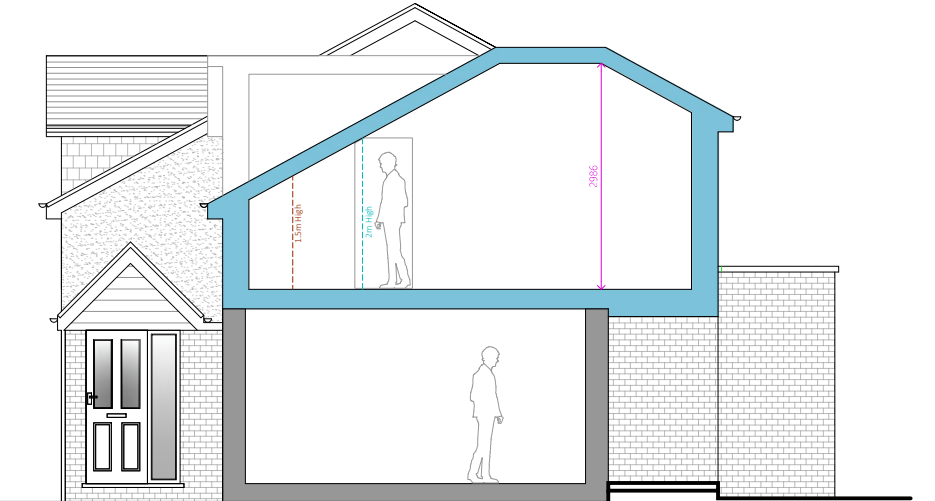
9 Proposed Side Section
