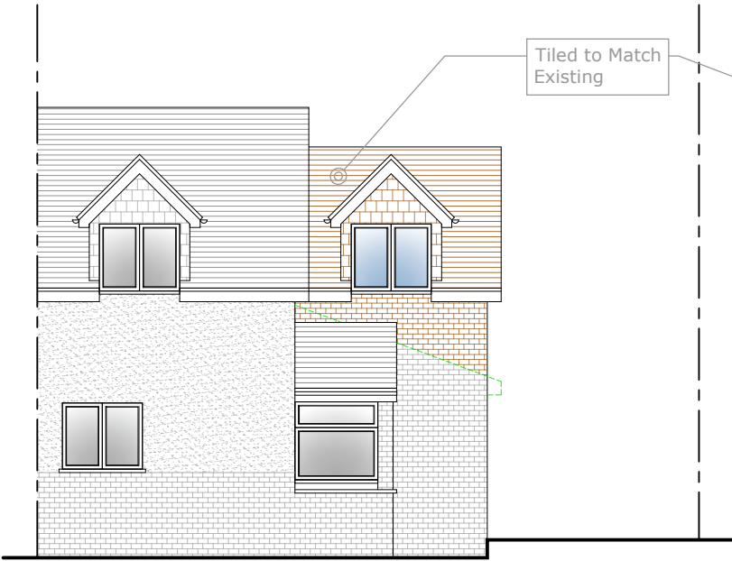
4 Proposed Front Elevation
