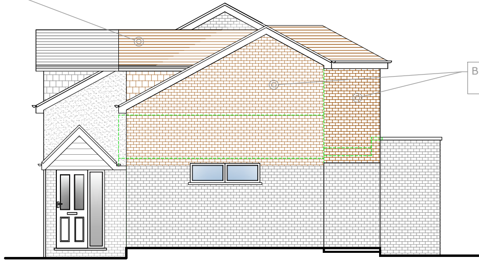
5 Proposed Side Elevation
