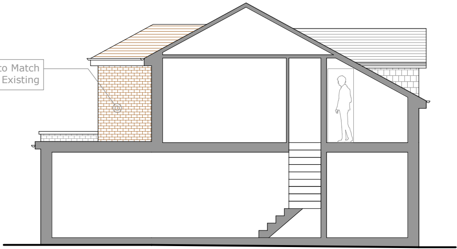
6 Proposed Side Section
