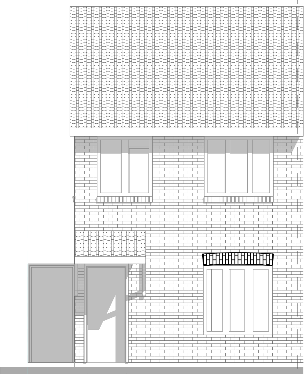
Front Elevation (1)
