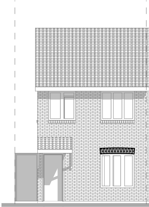
Front Elevation (1)
