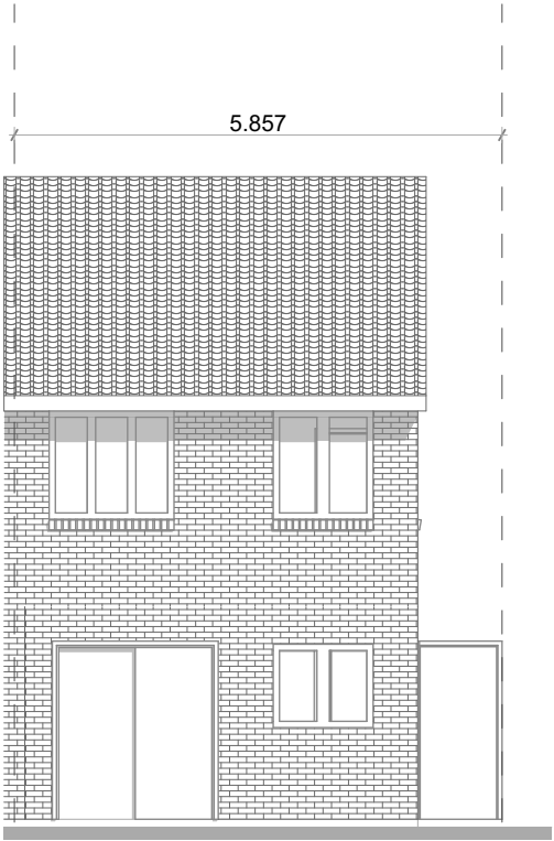
Rear Elevation (1)
