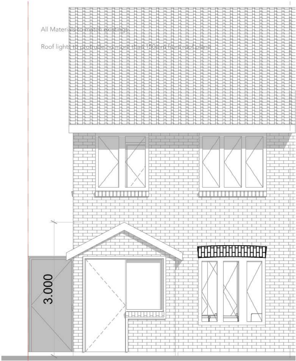
Front Elevation
