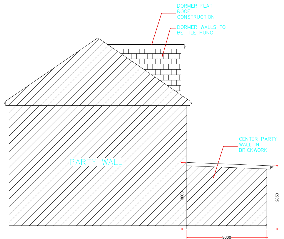
SIDE ELEVATION
