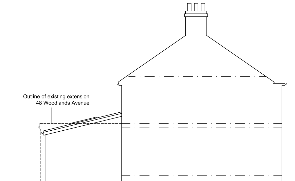
PROPOSED SECTIONAL SIDE ELEVATION
