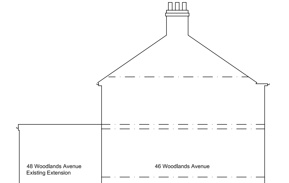
EXISTING SECTIONAL SIDE ELEVATION
