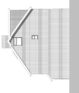
East elevation - Existing 1 : 100
