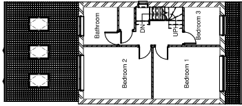
00 - Proposed 1 : 100
