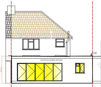
PROPOSED REAR ELEVATION NO ALTERATION SCALE: 1/100 @ A1
