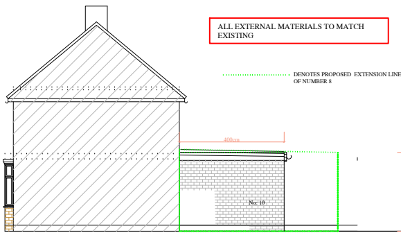
PROPOSED LEFT SIDE ELEVATION
