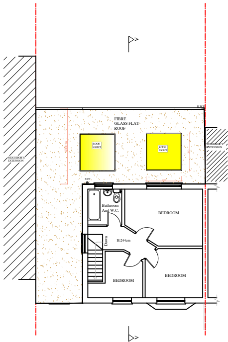
PROPOSED FIRST FLOOR PLAN SCALE: 1/100 @ A1
