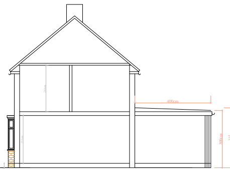
PROPOSED SECTION A-A
