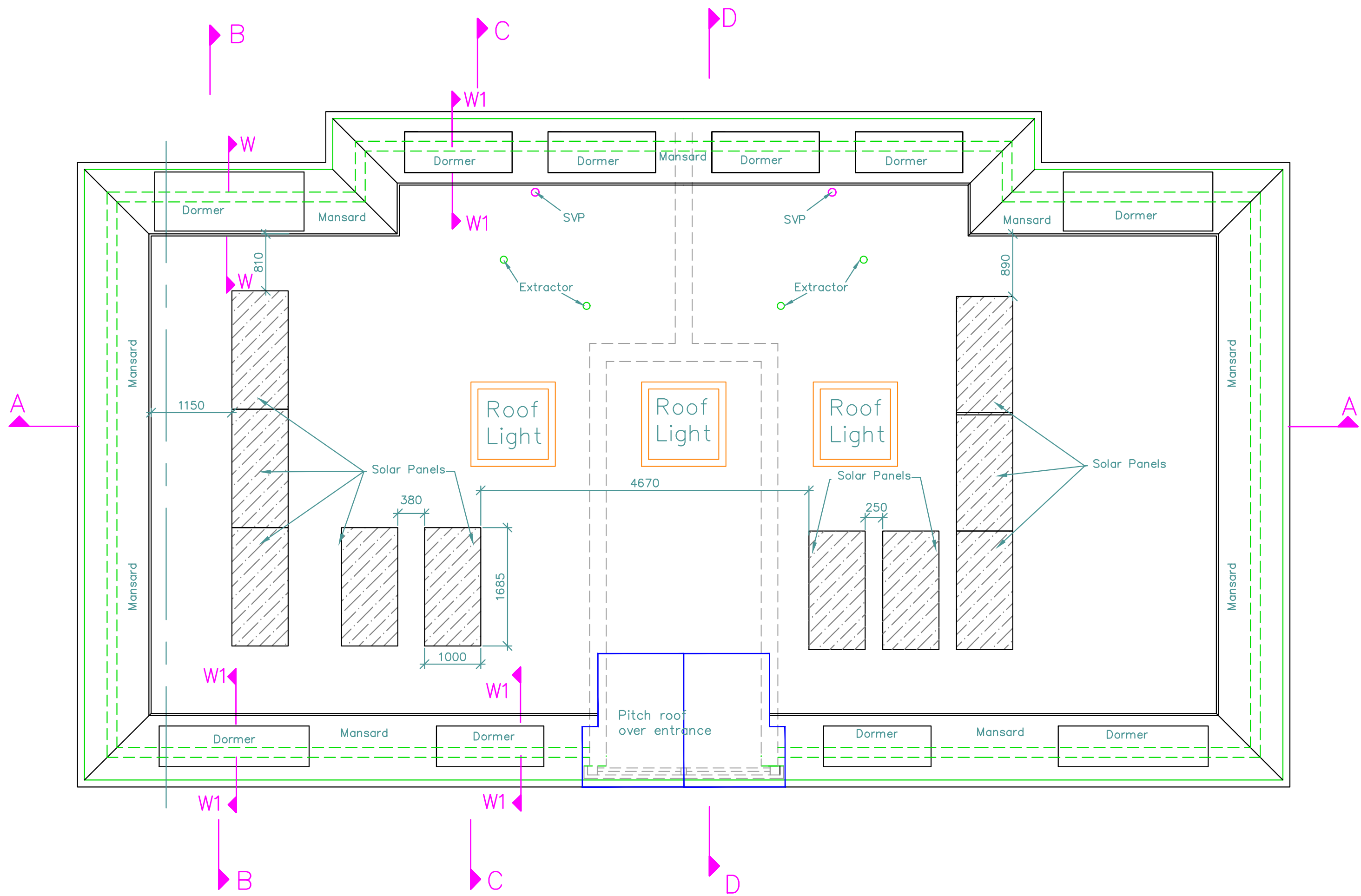
Roof Layout
