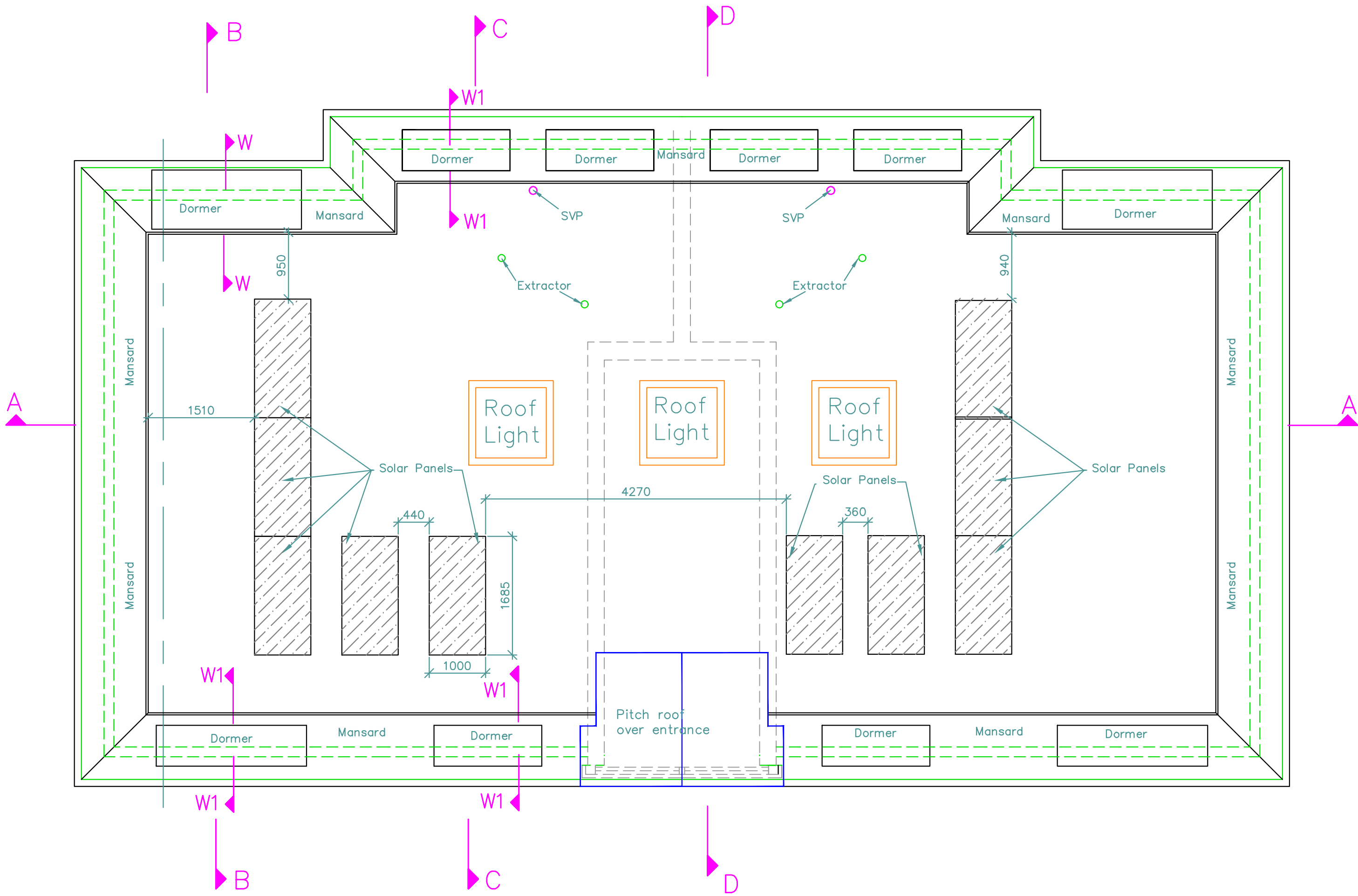
Roof Layout
