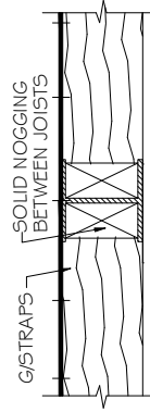
FLOOR JOISTS/ SB1
