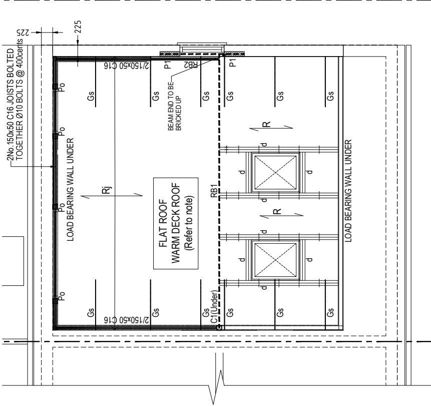
ROOF PLAN
