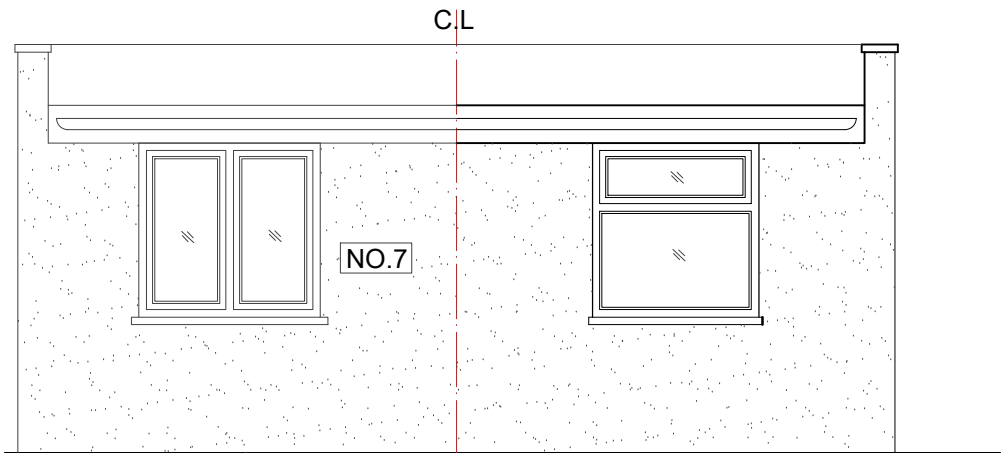
05 - REAR ELEVATION
