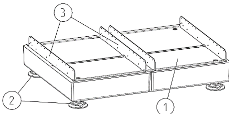
Figure 385 – New FM Duo machine base
