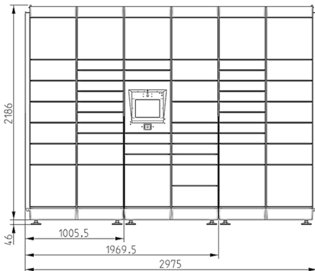
Figure 386 – External dimensions - front of the New FM Duo machine W1UCB + CB
