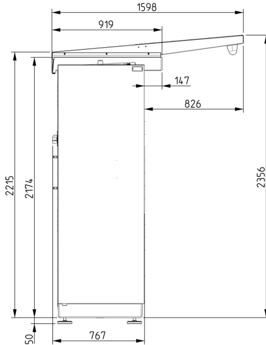
Figure 97 - External dimensions – Automatic Parcel Station side
