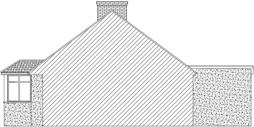
EXISTING RIGHT SIDE ELEVATION
