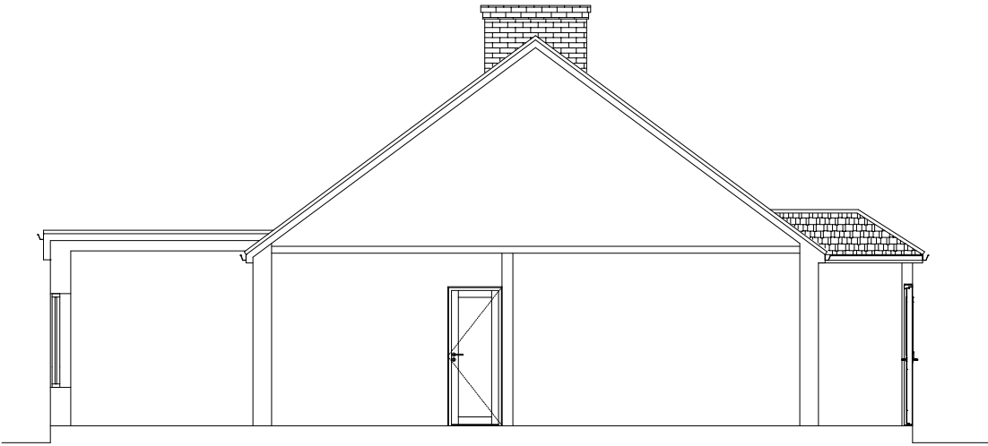
EXISTING SECTION
