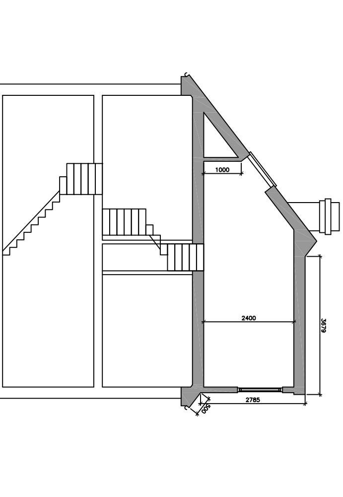
PROPOSED SECTION
