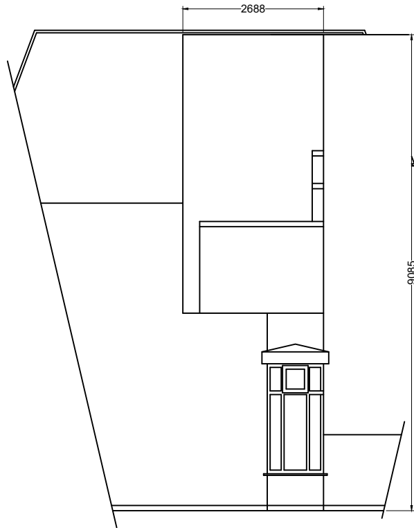
Existing Side Elevation (East) (1:100)
