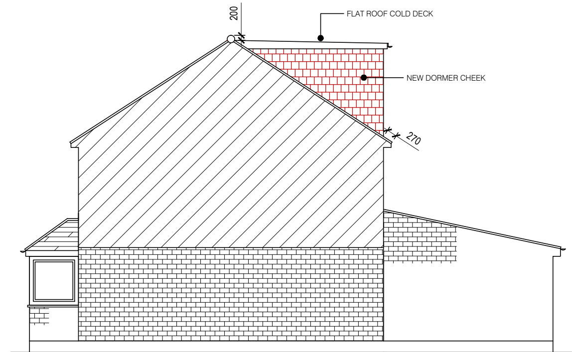
PROPOSED - SIDE ELEVATION (R/H)
