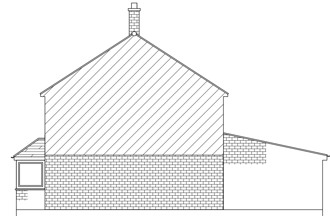
EXISTING - SIDE ELEVATION (R/H)
