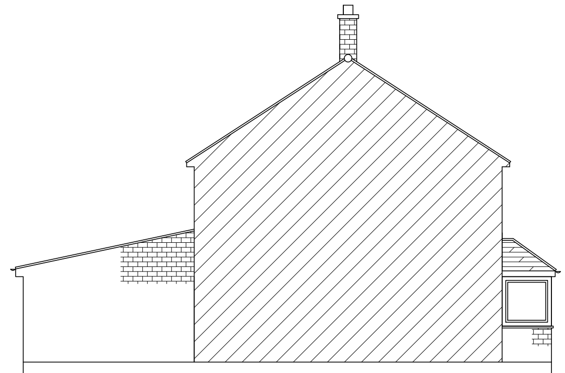
EXISTING - SIDE ELEVATION (L/H)
