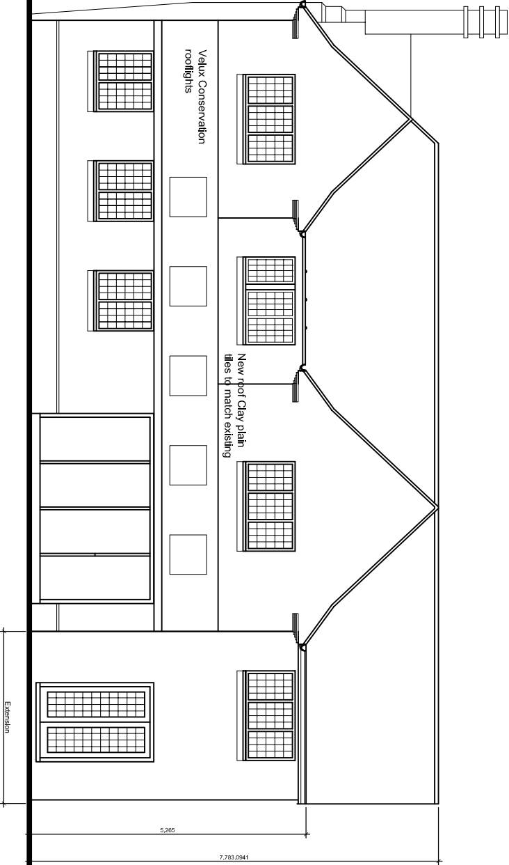
Garden elevation
