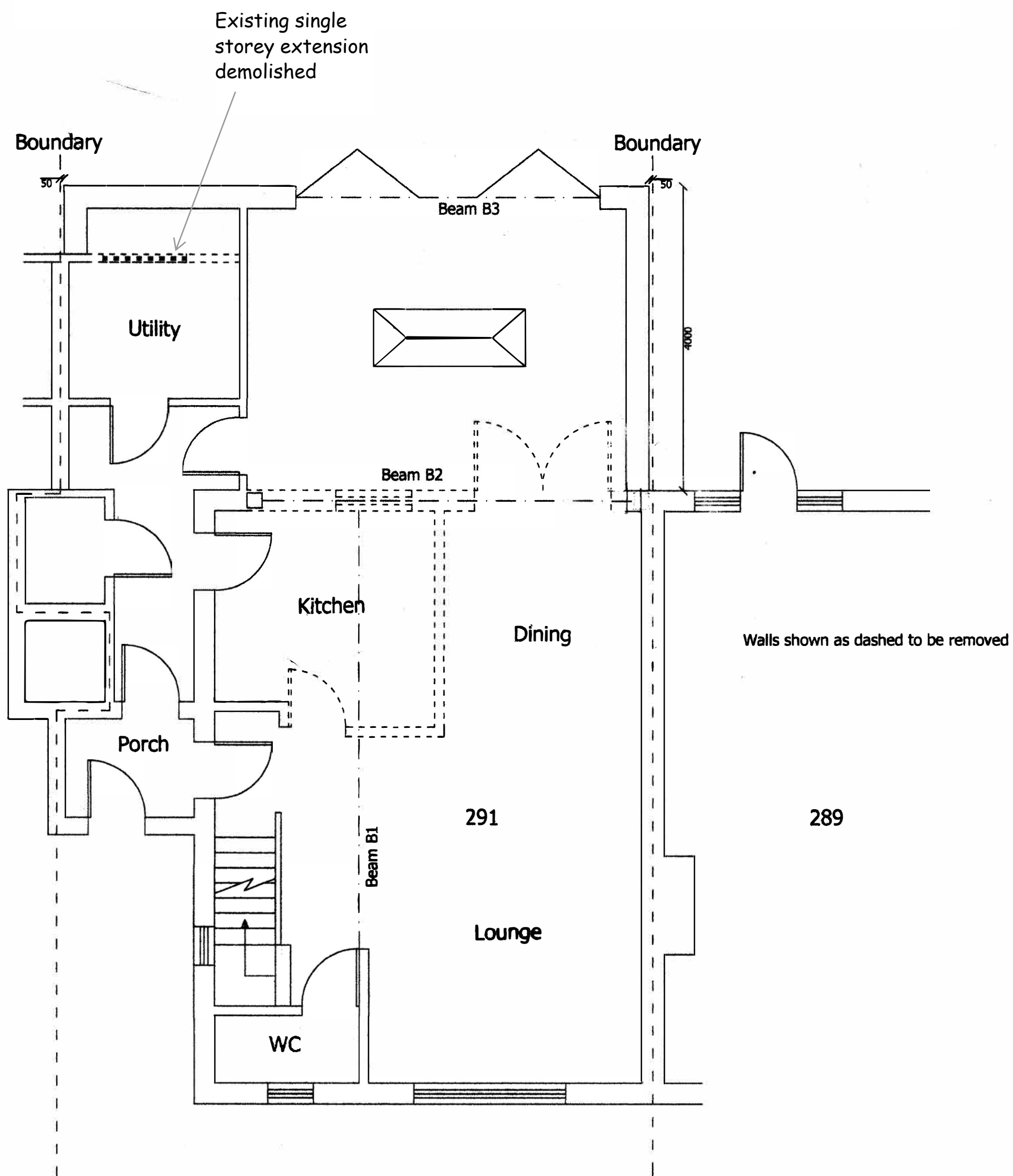
Proposed Ground Floor Plan 1:50@A3
