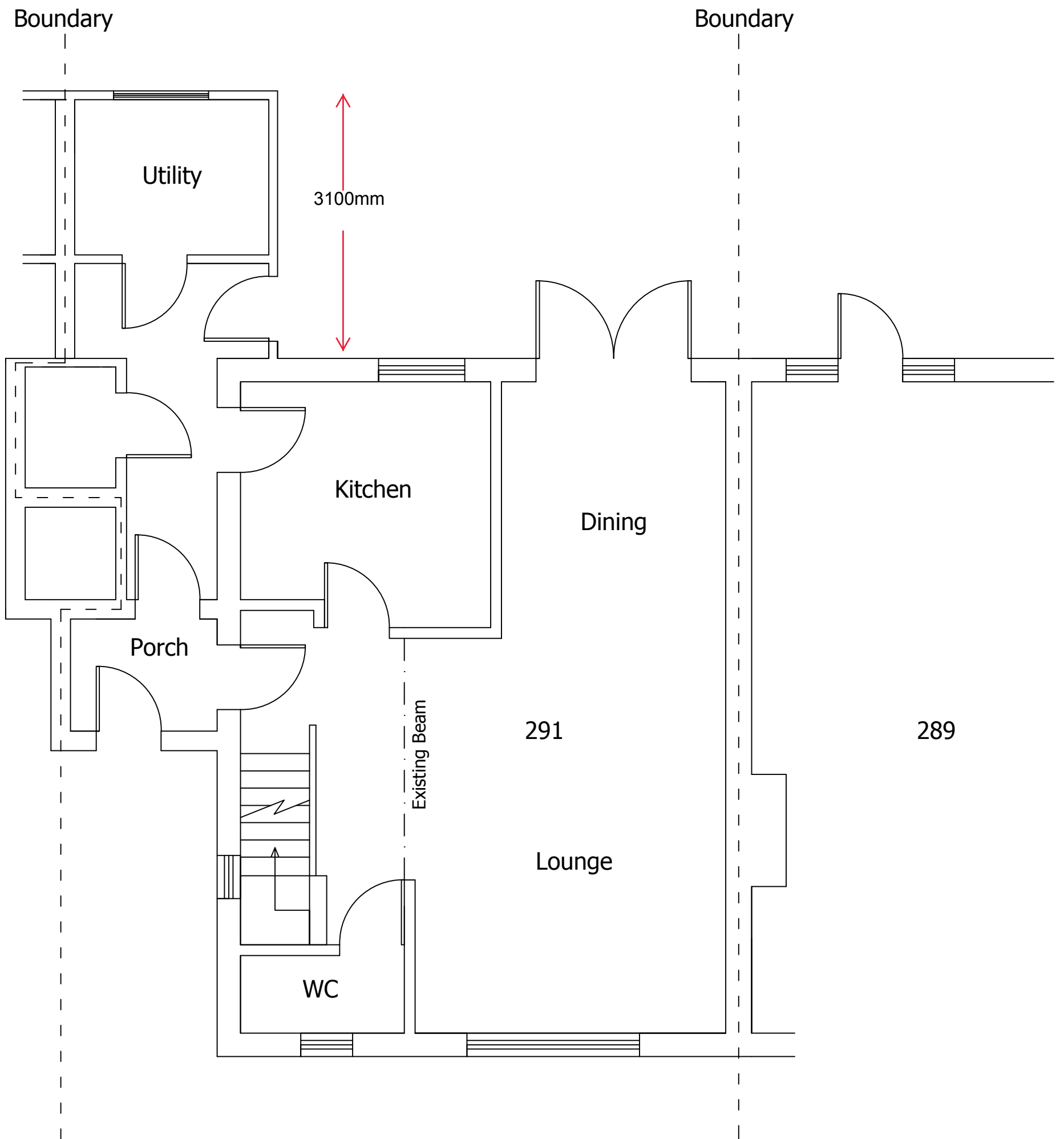
Existing Ground Floor Plan 1:50@A3
