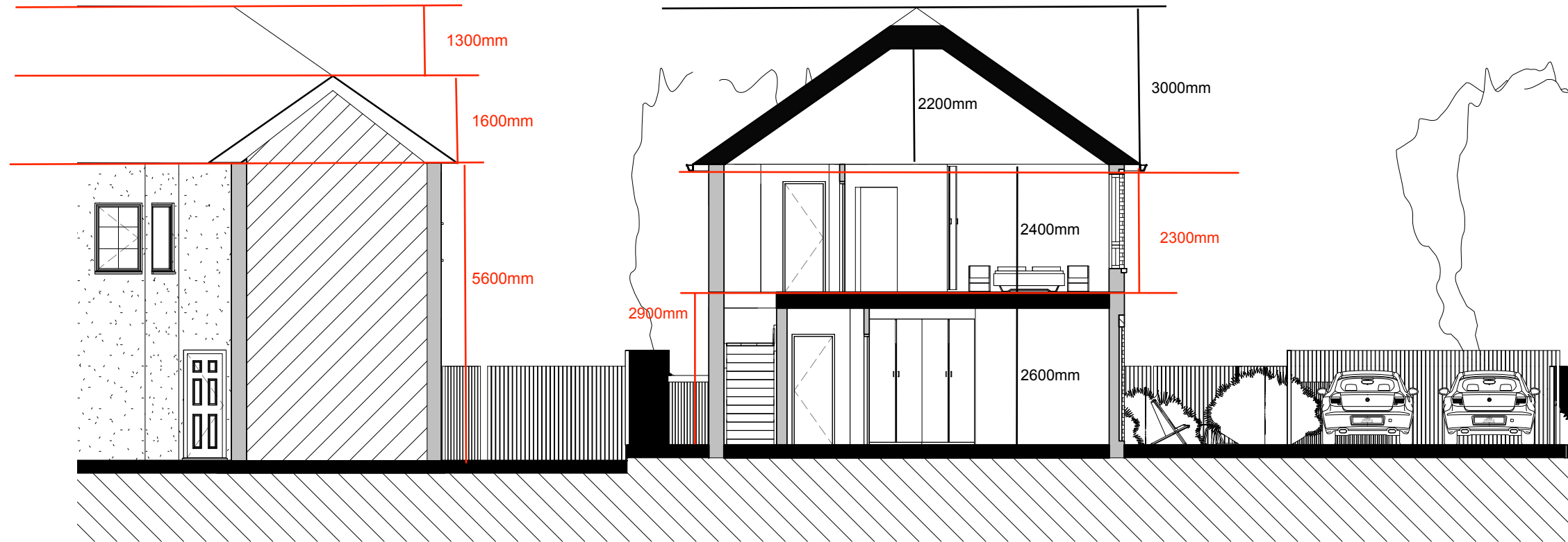
SECTION AA 1:100
