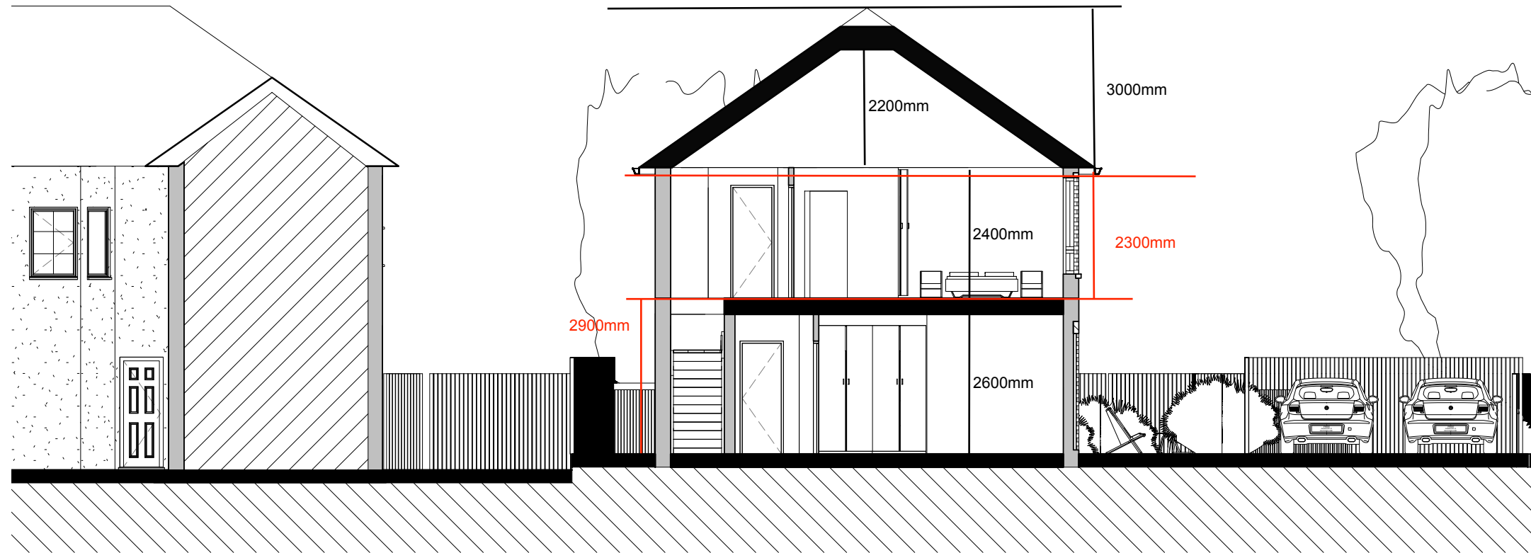
SECTION AA 1:100
