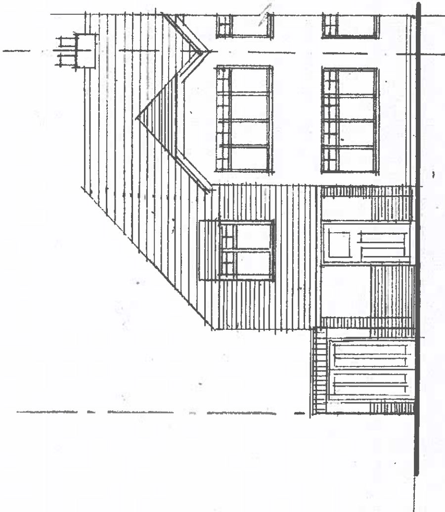
STREET ELEVATION
